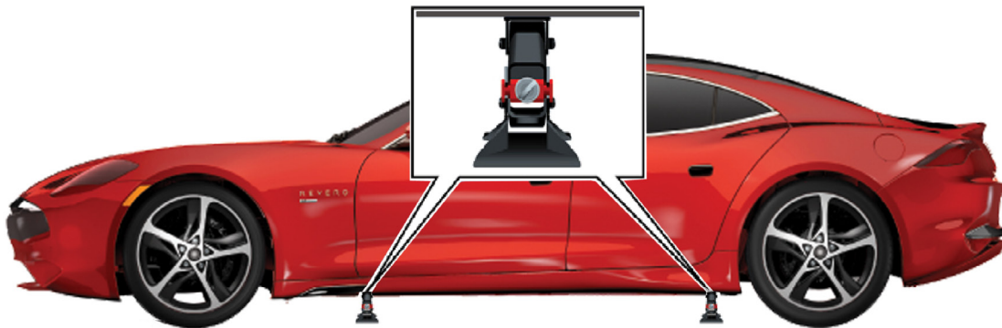
Stabilization and lifting locations (side view)
